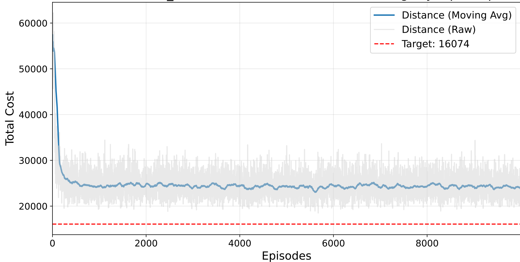
Final RANDOM_SEARCH Masked AutoRL-SOP Training - ry48p.2.sop
